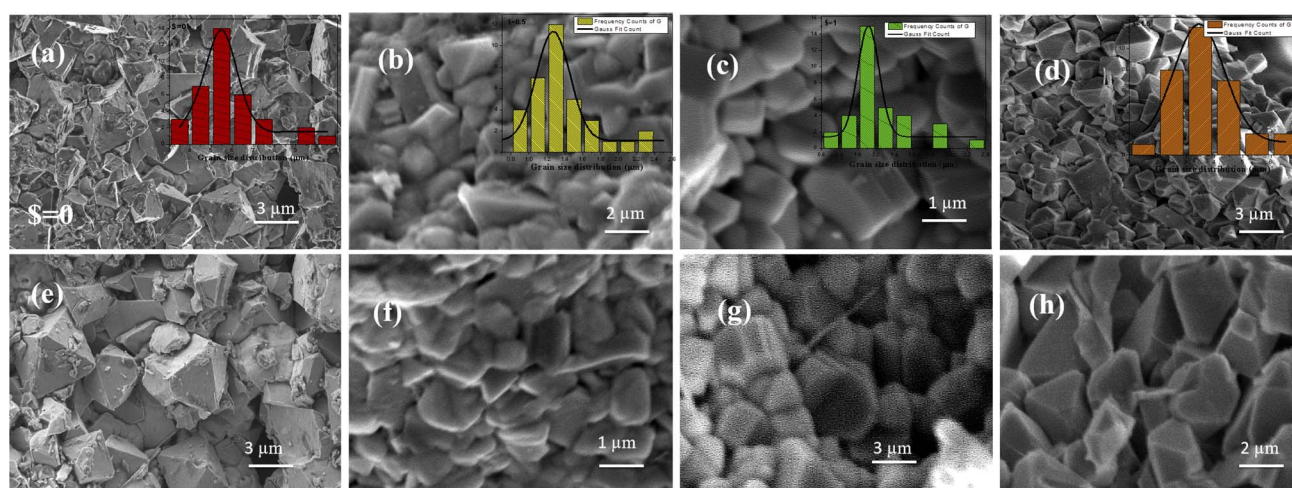
Fig. 3 Microstructural study through FEG-SEM images (insets represent the grain size distribution): (a) and (e) 0.5CNF–0.5BZT, (b) and (f) 0.5CNF–0.5BZT–0.5%GO, (c) and (g) 0.5CNF–0.5BZT–1%GO and (d) and (h) 0.5CNF–0.5BZT–1.5%GO.
