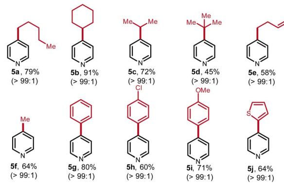
Fig. 3 Scope of Grignard reagents. The yields refer to the isolated yields of pure compounds. The ratios were determined by ^1\text{H} NMR and GC-MS. Due to the low boiling points, the yields of 5c and 5f were determined by ^1\text{H} NMR. Please see ESI† for experimental details.
