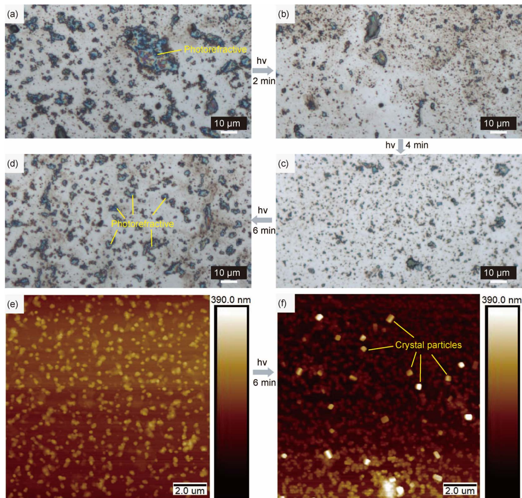
Fig. 4 Crystalline structure via high-level self-assembly. Morphology for aqueous HB-CyD solution with a higher concentration (1 mg mL -1 ) under optical microscope observation (a) before and after irradiation for (b) 2 min, (c) 4 min, and (d) 6 min, respectively. The photorefractive phenomenon can be seen from both the initial and the photostationary states. AFM images (height mode) of HB-CyD prepared from the aqueous solution with a lower concentration (0.1 mg mL -1 ) (e) before and (f) after UV irradiation.
