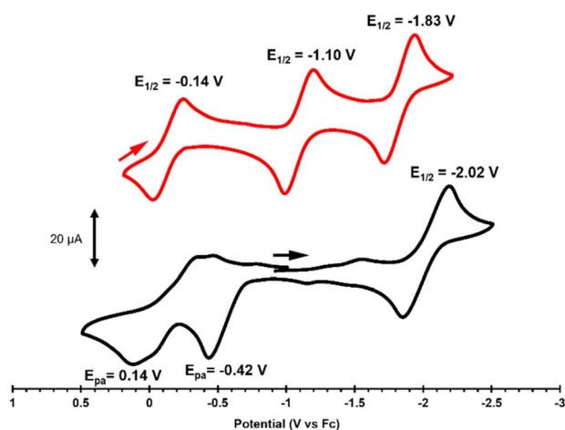
Fig. 3 Cyclic voltammograms of 1 (bottom, black) and 2 (top, red) in 0.1 M [ n\text{-Bu}_4\text{N} ][PF 6 ] solution (scan rate = 100 mV s -1 ). All potentials are referenced to Fc/Fc + .
