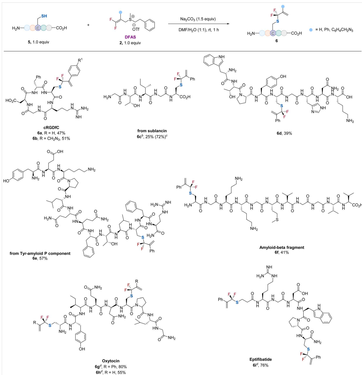
Scheme 2 Late-stage S - gem -difluoroallylation of unprotected cysteine-containing peptides with DFASs 2 . a Reaction conditions: 5 (0.02 mmol, 1.0 equiv.), 2 (1.0 equiv.), \text{Na}_2\text{CO}_3 (1.5 equiv.), \text{H}_2\text{O} (1 mL), DMF (1 mL), rt, 1 h. b The reaction was carried out on a 0.04 mmol scale. c 19 F NMR yield. d (i) 5 (0.02 mmol, 1.0 equiv.), TCEP·HCl (1.5 equiv.), \text{Na}_2\text{CO}_3 (3.0 equiv.), \text{H}_2\text{O} (1 mL), DMF (1 mL), rt, 1 h; (ii) 2 (2.0 equiv.), rt, 1 h.
