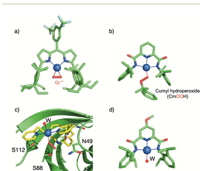
Fig. 6 Selected crystallographic structures of recently described mononuclear copper–oxygen adducts. a) \eta^2 -superoxo based on the ^E\mathbf{M}\mathbf{i}\mathbf{n}\mathbf{d}\mathbf{L} ligand. 83 Hydrogen atoms were omitted for clarity; b) The anion [(L)Cu(OOCm)] - based on the bis(arylcarboxamido)-pyridine ligand. 85 Hydrogen atoms and the Et 4 N + counter ion were omitted for clarity; c) \eta^1 -Hydroperoxido complex in an artificial enzyme based on a streptavidin scaffold: [(biot-et-dpea)Cu II (OOH)(OH 2 )] + c Sav; 86 d) High-valent [(L)CuOH] species based on the bis(arylcarboxamido)-pyridine ligand (W as deprotonated water ligand). 87
