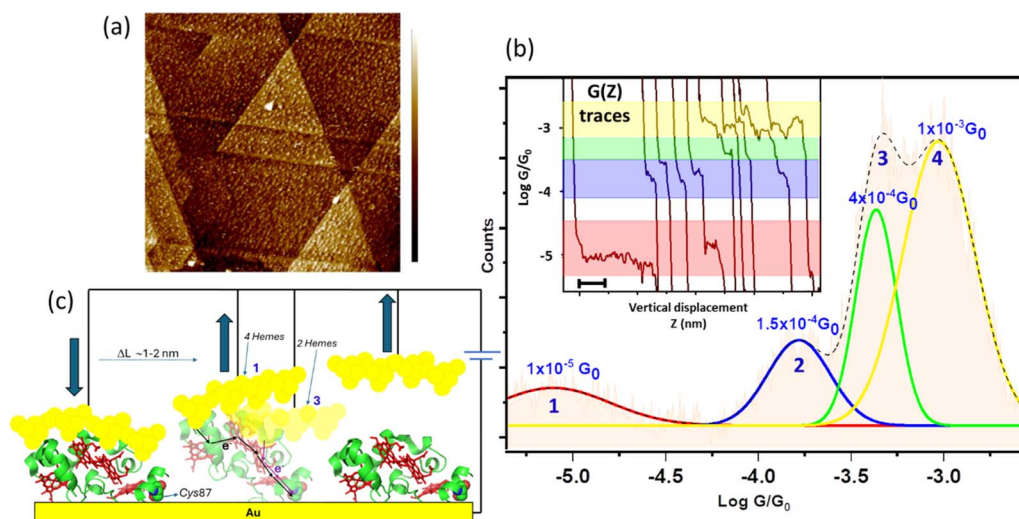
Fig. 2 (a) 400 \times 400 \text{ nm}^2 STM image of Cys87-modified STC proteins on Au surface. Each bright spot in the image corresponds to an individual STC. Characteristic triangulated atomically flat Au(111) terraces are >200 nm wide. Colour legend on the right spans from 0 to 1.2 nm. (b) Semi-log scale conductance ( G ) histogram accumulating 1350 selected G(z) traces (representative ones in the inset) at an applied 200 mV bias voltage. Individual Gaussian fits of the peaks (coloured solid lines) are used to extract the maxima values corresponding to the average conductance of each of the four features. The dotted line (—) is a cumulative plot including all the Gaussian peaks for visual guidance. Figure inset shows illustrative individual G(z) traces displaying plateau features used to build the 1D histogram. The X-axis scale bar at the left-bottom corner corresponds to 0.6 nm. (c) Pictorial representation of the STM break-junction process showing two possible scenarios leading to the low G (peak 1 in (b)) and high G (peak 3 in (b)) involving 4 and 2 hemes in the pathway, respectively, where STM tip asperities (represented as yellow balls) contact different points of the protein surface during different pulling cycles of the anchored ( via Cys(thiol)) STC on the Au substrate.
