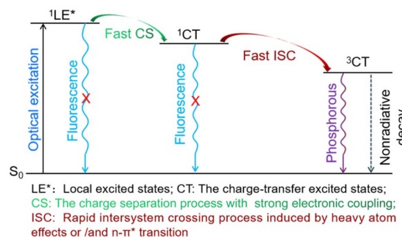
Fig. 10 The schematic illustration of the probable emission mechanism of PhSeDB emitters.
