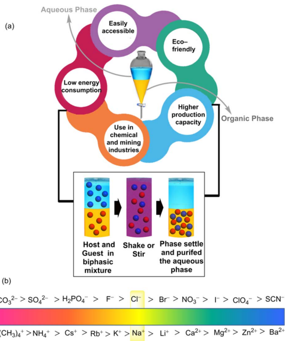
Fig. 1 (a) Schematic illustration of the liquid-liquid extraction process. (b) Conceptual sketch of the Hofmeister series.
