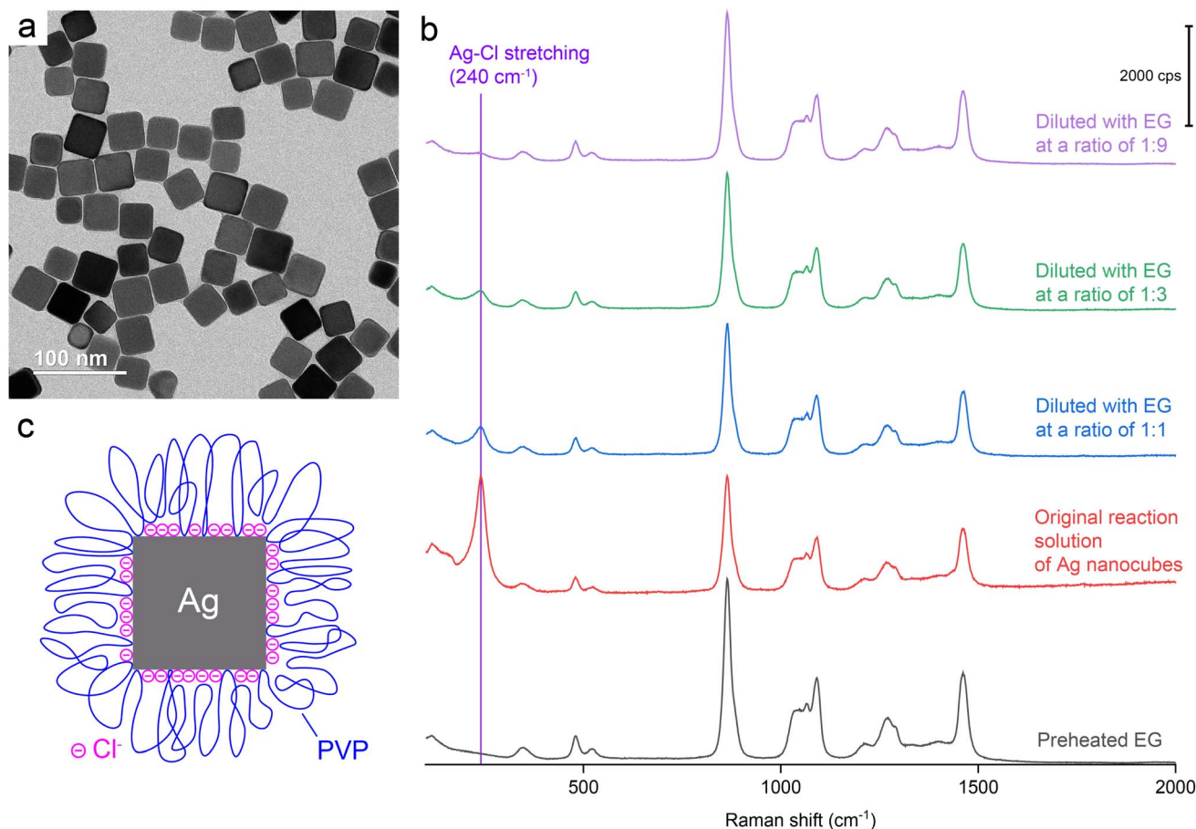
Fig. 1 (a) A typical TEM image of the Ag nanocubes. (b) Raman spectrum of EG (preheated at 150 \text{ }^\circ\text{C} for 1 h) and SERS spectra recorded from the original reaction solution of Ag nanocubes and after it had been diluted with preheated EG at various ratios. (c) A model detailing the native surface of a Ag nanocube suspended in the original reaction solution.
