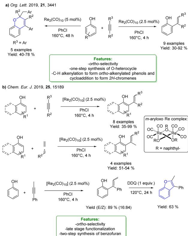
Scheme 62 Re-catalysed ortho -alkenylation of phenols with alkynes and cyclization to 2 H -chromene. 181,182
