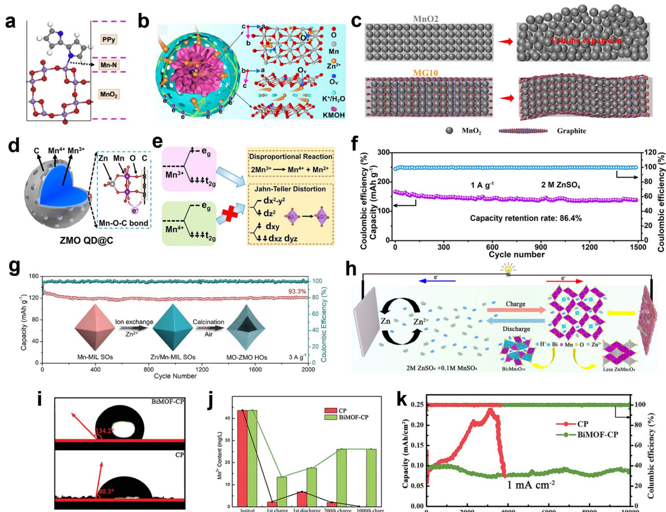
Fig. 11 Strategy for rational composite design based on one-electron transfer reaction. (a) Optimal configuration of the disordered \text{MnO}_2 surface covered by PPy. Reproduced with permission. 113 Copyright 2020, Elsevier. (b) Schematic illustration of the Zn-ion/electron transport in \text{KMOH@C} with oxygen vacancies. Reproduced with permission. 138 Copyright 2021, Elsevier. (c) Schematic illustration of the volume change in \text{MnO}_2 and \text{MnO}_2/\text{graphite} . Reproduced with permission. 116 Copyright 2020, Elsevier. (d) Illustration of the Mn valence state distribution in \text{ZMO QD@C} . (e) Mechanism for the structural stability of \text{ZMO QD@C} . (f) Long-term cycle test. (d)–(f) Reproduced with permission. 139 Copyright 2022, Wiley-VCH. (g) Cycling performance of hetero-structured \text{Mn}_2\text{O}_3\text{--ZnMn}_2\text{O}_4 hollow octahedrons. Reproduced with permission. 146 Copyright 2021, Wiley-VCH. (h) Schematic diagram showing the effects of bismuth in manganese-based ZIBs. Reproduced with permission. 147 Copyright 2021, the American Chemical Society. (i) Contact angle tests of \text{BiMOF-CP} and \text{CP} samples. (j) Element analysis of deposited \text{Mn}^{2+} in 2\text{ M ZnSO}_4/0.2\text{ M MnSO}_4 aqueous electrolyte during cycling of \text{BiMOF-CP} and \text{CP} . (k) Cycling performance of \text{BiMOF-CP} and \text{CP} . (i)–(k) Reproduced with permission. 148 Copyright 2023, Wiley-VCH.
