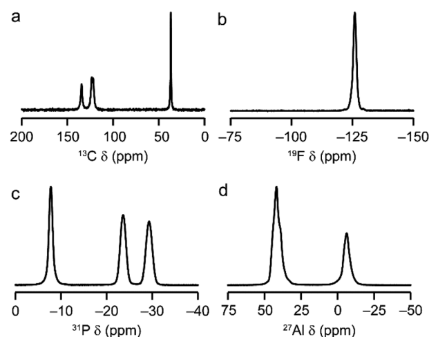
Fig. 2 Solid-state NMR spectra of as-made AlPO-34(mim): (a) ^{13}\text{C} (9.4 T, 12.5 kHz CP MAS), (b) ^{19}\text{F} (14.1 T, 50 kHz MAS), (c) ^{31}\text{P} (9.4 T, 14 kHz MAS), (d) ^{27}\text{Al} (9.4 T, 14 kHz MAS). Further experimental details are given in Table S1.†
