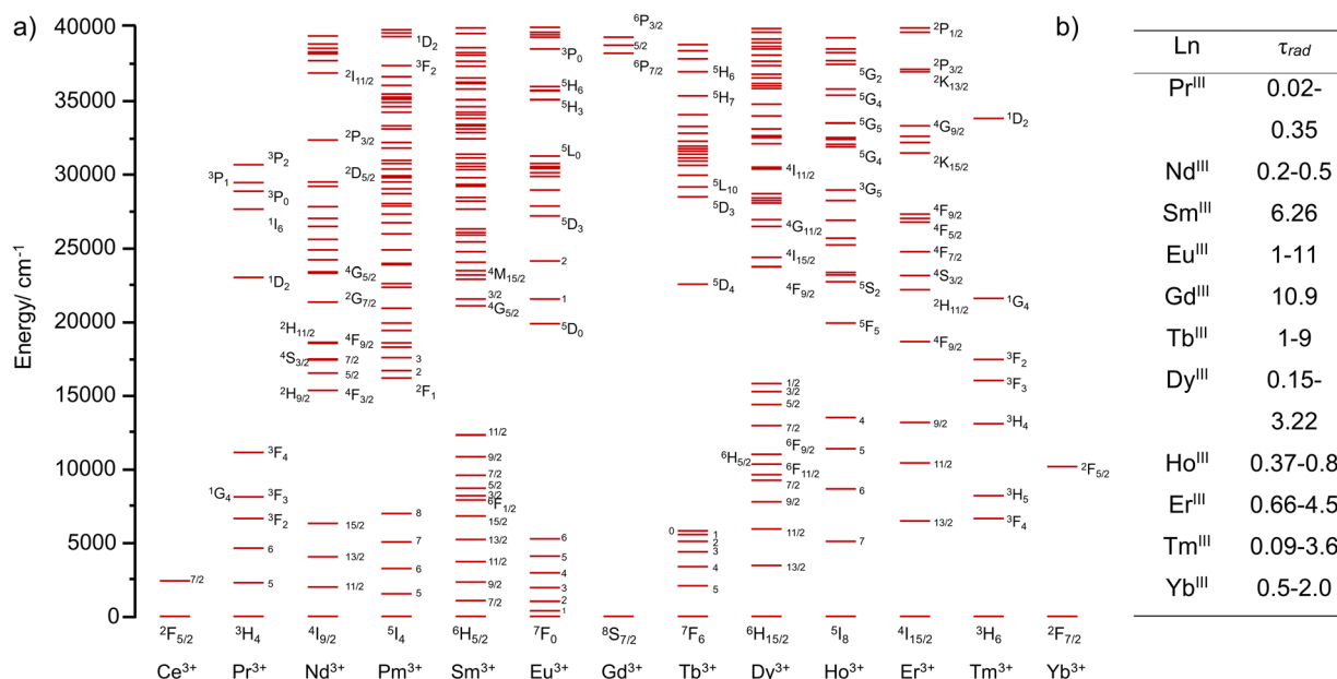
Fig. 1 (a) Calculated energy levels of Ln(III) 22 and (b) ranges of radiative lifetimes \tau_{rad} for different Ln(III) ions (in ms). 23
