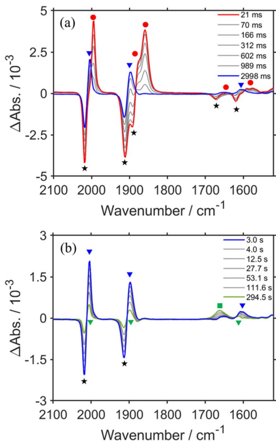
Fig. 1 TR-IR spectra of \text{CO}_2 saturated DMSO-TEOA (5 : 1 v/v) solution containing \text{RuC}_2\text{Re} (1.0 mM) and BIH (0.1 M) (a) from 21 ms to 3.0 s and (b) from 3.0 s to 5.0 min after pulsed excitation at 532 nm. A total of 50 loops of spectra using the two samples were averaged for the final data.
