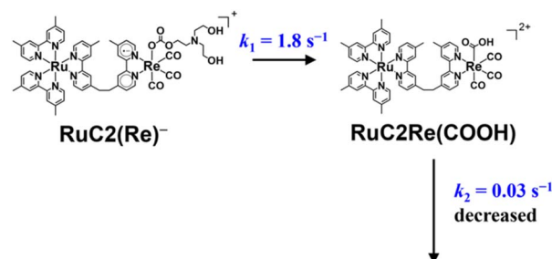
Scheme 2 Conversion reaction from \text{RuC}_2(\text{Re})^- to \text{RuC}_2\text{Re}(\text{COOH}) and the rate constant of the following process.
