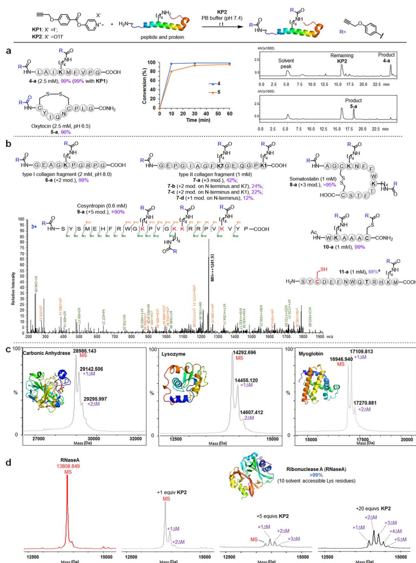
Fig. 3 Chemo-selective amidation of pyridinium esters on lysine residue sites in peptides and proteins. (a) Model reactions between KP2 and peptides, the inserted chart exhibits HPLC determined conversion versus time plot, and the LC traces of directly analyzing of reaction mixtures of peptide 4 and 5 . Standard conditions for peptide: KP2 (10 mM), peptide (indicated concentration in parenthesis) and in PB buffer (pH 7.4, 50% MeCN) for 1 hour at rt. (b) Range of bioactive peptides and protein fragments. “ +n mod.” refers to the number of modifications on the amino groups. (c and d) Modification efficiency of KP2 on proteins by MALDI-TOF analysis. \Delta m = 158 Da. Standard conditions for protein: KP2 (50 \mu M, 250 \mu M and 1000 \mu M, respectively), protein (50 \mu M) and in PBS (pH 7.4) for 1 hour at 37 ^{\circ} C. a 20 mM DTT was added after amidation.
