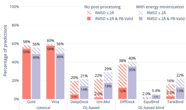
Fig. 5 Comparative performance of docking methods with post-docking energy minimisation of the ligand (while keeping the protein fixed) on the PoseBusters Benchmark set. The striped bars show the share of predictions of each method that have an RMSD within 2 Å of the crystal pose and the solid bars show those predictions which in addition pass all PoseBuster tests and are therefore PB-valid. Post-docking energy minimisation significantly improves the relative physical plausibility of the DL-based methods' predictions. This indicates that force fields contain docking-relevant physics which is missing from DL-based methods.
