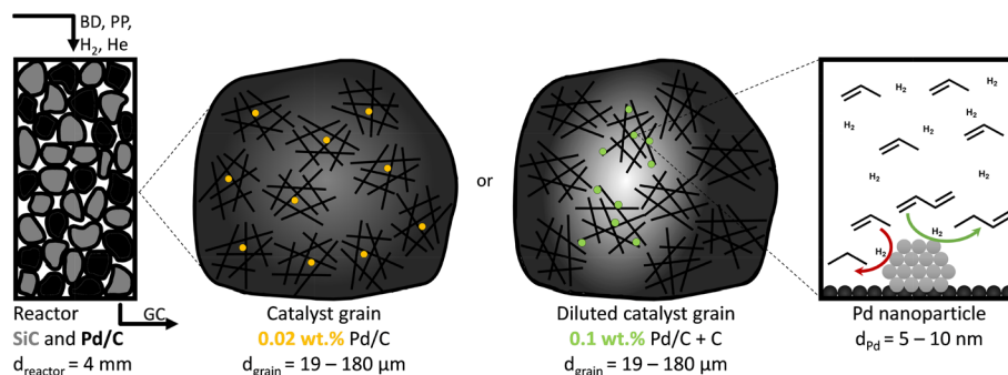
Fig. 1 Schematic representation of selective hydrogenation reactor at different length scales. From left to right: 4.0 mm internal diameter fixed reactor with inlet gas mixture of 0.3% butadiene (BD), 30% propylene (PP), 20% hydrogen and 49.7% helium. Pd/C catalyst grains (black) are mixed with nonporous and inert SiC particles (grey). Reactant and product concentrations are analysed by on-line gas chromatography (GC). Middle: catalyst grains with non-diluted 0.02% Pd/C or 0.1% Pd/C diluted in GNP to achieve equal Pd weight loading in each reactor. The greyscale schematically indicates the reactant concentration in the grains during catalysis, as it is converted over the active Pd nanoparticles, but not over the inert carbon dilutant. Right: Selective hydrogenation of butadiene over Pd nanoparticles, in an excess of hydrogen and propylene. Drawings not to scale.
