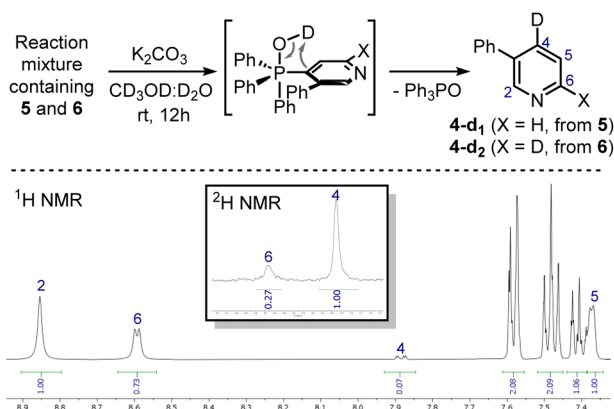
Scheme 4 Deuterodephosphination of the 5/6 mixture (top) and 1 H NMR and 2 H NMR spectra (CDCl 3 , 400 MHz) of the isolated mixture of 4- d 1 /4- d 2 (bottom). Deuterium incorporation was determined by the relative integration of the signals of hydrogens on the pyridine ring.
