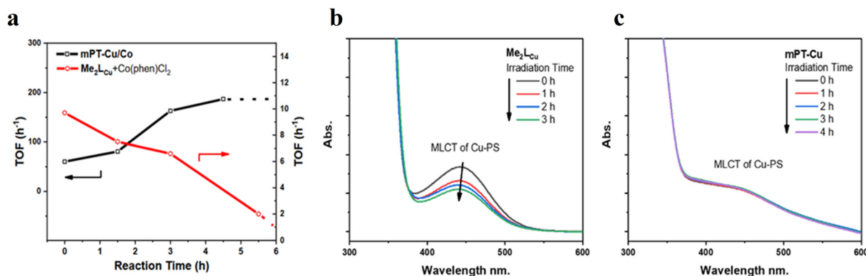
Fig. 18 (a) Time-dependent TOF curves of mPT-Cu/Co (black) and \text{Me}_2\text{L}_{\text{Cu}} + \text{Co}(\text{phen})\text{Cl}_2 (red) in the first 5 h of photocatalytic HER, where \text{Me}_2\text{L}_{\text{Cu}} is [\text{Cu}(\text{Me}_2\text{PT})(\text{dppe})]\text{PF}_6 , and UV-vis absorption changes for \text{Me}_2\text{L}_{\text{Cu}} (b) and mPT-Cu (c) under catalytic HER conditions ( \text{N}_2 atmosphere, \text{CH}_3\text{CN} : \text{AcOH} = 1.97 : 0.03 ) at different irradiation times. Adapted with permission from ref. 75. Copyright 2020, the American Chemical Society.
