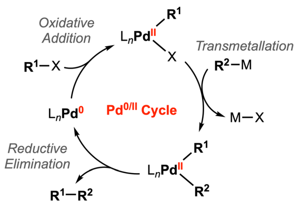
Fig. 3 General catalytic cycle for Pd-catalyzed cross-coupling reactions. 16
