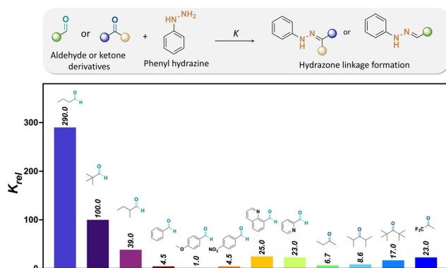
Fig. 14 Relative formation rates ( K_{\text{rel}} ) of hydrazones from a selected set of aldehydes and ketones at pH 7. 127 The relative reaction rates refer to the hydrazone formation between either aldehyde or ketones and phenylhydrazine [ K_{\text{rel}}(4\text{-methoxybenzaldehyde}) = 1 ]. 67
