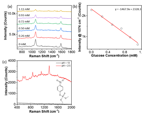
Fig. 8 (a) Glucose detection using 4-MCBA with PAA-grafted AgNPs at concentrations of 0 \text{ mM} to 1.11 \text{ mM} of glucose in addition to 0.5 \text{ M H}_3\text{PO}_4 solution. (b) Plotting the peak intensity of 4-MCBA at 1074 \text{ cm}^{-1} vs. glucose concentrations of 0 \text{ mM} to 1.11 \text{ mM} . (c) Detection of methyl parathion using PAA-grafted AgNPs at a concentration of 17 \text{ ppm} after adding \text{H}_3\text{PO}_4 .
