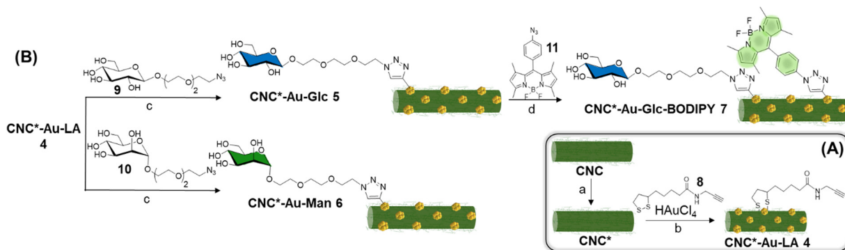
Scheme 1 (A) Synthesis of CNC*-Au-LA 4 . Reaction conditions: a. Sulfur trioxide pyridinium complex, dimethyl sulfoxide, 4 h, 25 °C; b. \text{HAuCl}_4 , \text{NaBH}_4 , water:methanol (1: 9), and 8 . (B) Synthesis of CNC*-Au-Glc 5 , CNC*-Au-Man 6 , and CNC*-Au-Glc-BODIPY 7 . Reaction conditions for c and d: \text{CuSO}_4 , sodium ascorbate (water for c and DMF for d), overnight, room temperature.
