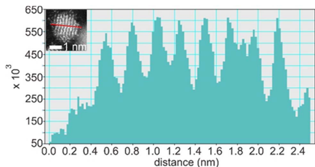
Fig. 8 Line profile through (111) planes (marked by a red line in the inset) of an Ag/Pt NP shown in the inset of the figure. Adapted with permission of ref. 61. Copyright 2021, the American Chemical Society.
