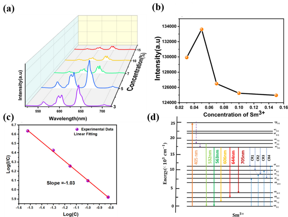
Fig. 6 (a) PL spectra of the \text{LSYW}:x\%\text{Sm}^{3+} phosphors, (b) plot of the intensity vs. \text{Sm}^{3+} concentration (c) linear fitting of \log(I/C) in terms of \log(C) . (d) The mechanism of the down conversion-based luminescence process in \text{Sm}^{3+} ions.
