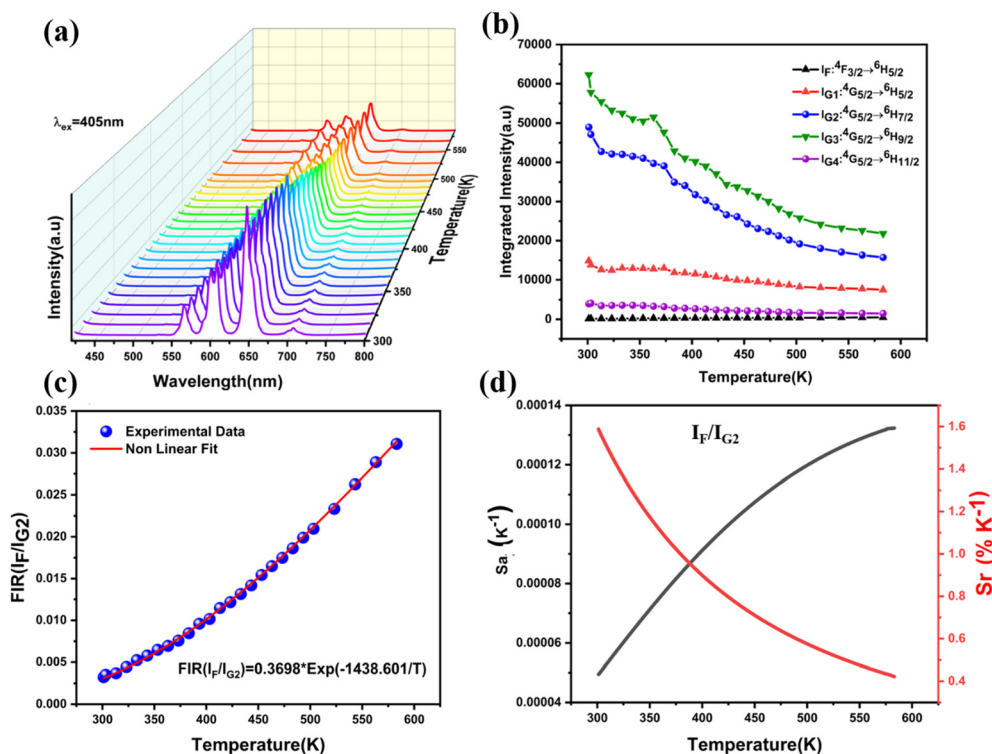
Fig. 7 (a) Down-conversion luminescence spectra of \text{LSYW}:0.05\%\text{Sm}^{3+} from 303 to 588 K, (b) the integrated intensities of various emission bands in 303–588 K. (c) The FIR ( I_F/I_{G2} ) of \text{LSYW}:5\%\text{Sm}^{3+} as function of temperature (303–588 K). (d) The absolute sensitivity and relative sensitivity of I_F/I_{G2} .
