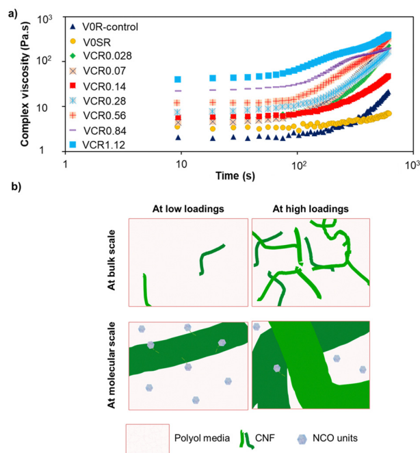
Fig. 1 (a) Complex viscosity of CNF/polyurethane resins dispersions; (b) schematic representation of the effect of CNF on the reactivity of CNF/polyol dispersions at low and high loadings.
