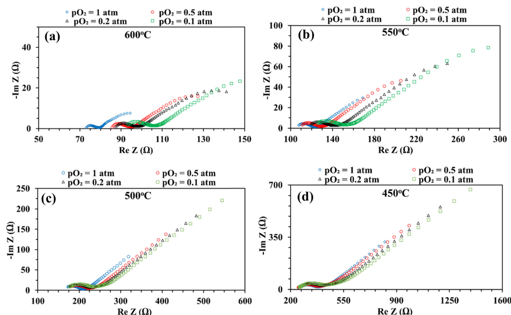
Fig. 8 Electrochemical impedance spectra (EIS) of an electrochemical cell with the patterned Ag working electrode and the PNC counter electrode in an O_2-N_2 mixture with p_{O_2} values of 1, 0.5, 0.2, and 0.1 atm at (a) 600, (b) 550, (c) 500, and (d) 450 °C, respectively.
