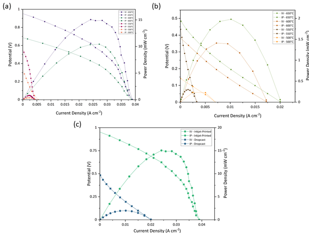
Fig. 9 IV and IP curves of (a) 100-layer inkjet-printed and (b) drop-cast full fuel cells with Ink (2) – Samba at 500–650 °C ( \text{H}_2 with 5 L min -1 and air with 12.5 L min -1 were supplied on the anode and cathode sides, respectively), and (c) comparison of inkjet-printed and drop-cast full fuel cells with Ink (2) – Samba at 650 °C.
