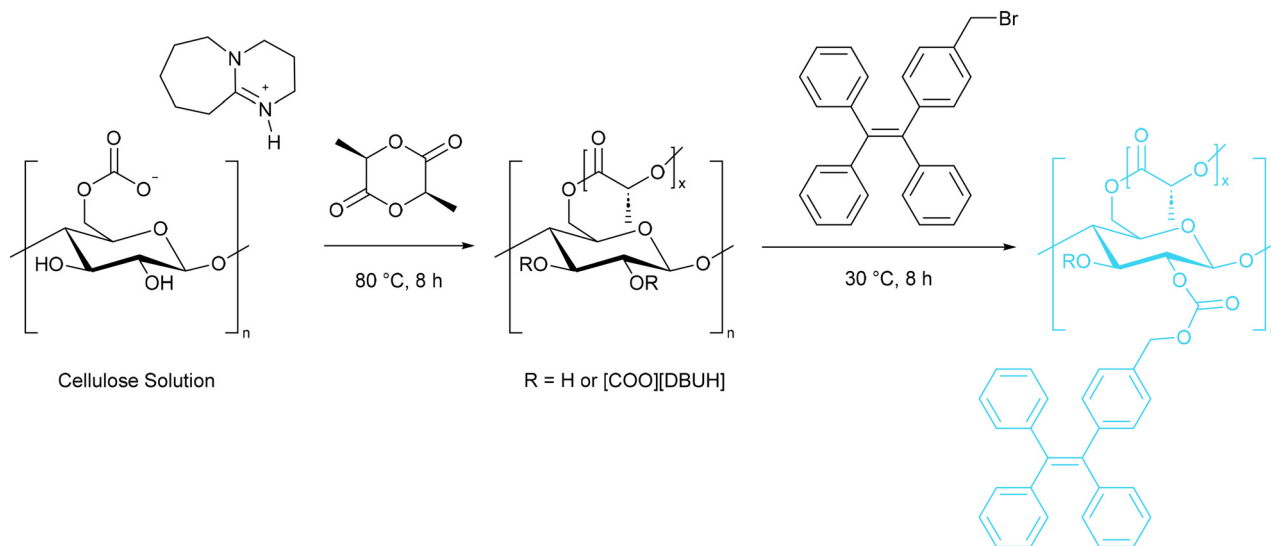
Scheme 19 The preparation of a fluorescent cellulose derivative with a poly(lactide) side chain. 91
