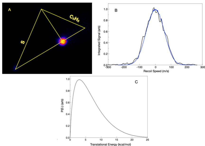
Fig. 6 (A) Velocity map image of the 99 u product, C 5 H 7 S, for the reaction of S( 3 P) with isoprene (Newton diagram superimposed) under a collision energy of 14.0 kcal mol -1 . (B) Total signal from the image in (A) projected onto the x-axis and transformed into a speed distribution (black). The simulated image using the velocity distribution is then projected to produce a profile (blue) that closely matches the observed one. (C) Total translational energy release ( P(E_T) ) extracted following analysis of the image in (A).
