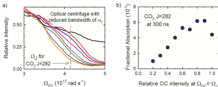
Fig. 6 (a) Optical centrifuge profiles with reduced bandwidth near the classical rotation frequency Q_J for \text{CO}_2 J=282 . (b) Transient IR absorption intensities for J=282 at t=300 ns as a function of the optical centrifuge relative intensity at Q_{\text{OC}} = Q_J .
