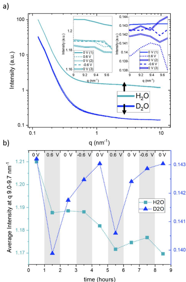
Fig. 3 SANS curves (a) and average SANS intensity in the q -range from 9.0\text{--}9.7 \text{ nm}^{-1} (b) for \text{H}_2\text{O} (light-blue rectangles) and \text{D}_2\text{O} (dark-blue triangles). The insets in (a) show the scattering intensity in the q -range of 9.0\text{--}9.7 \text{ nm}^{-1} .
