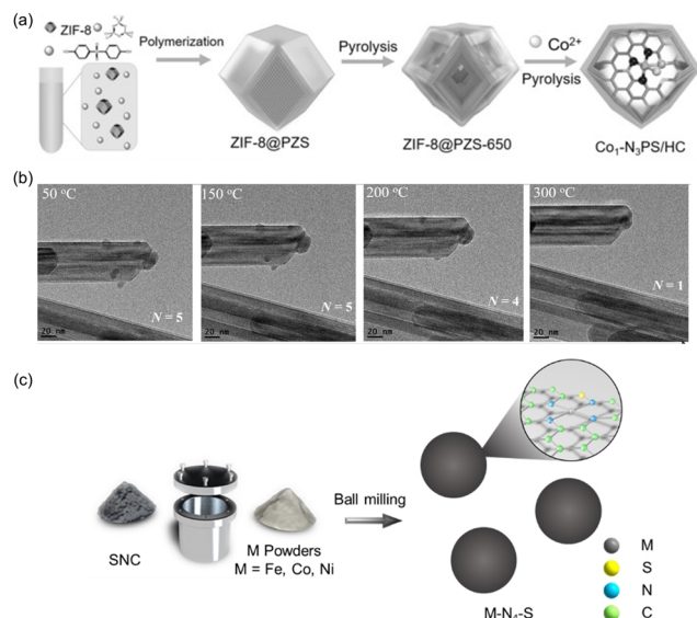
Fig. 9 (a) Schematic illustration of synthetic process of Co 1 -N 3 PS/HC. Reproduced with permission from ref. 192. Copyright 2020. Wiley-VCH. (b) TEM images of AgNP/MnO 2 at different temperature of 50, 150, 200, and 300 °C. Reproduced with permission from ref. 193. Copyright 2020. Wiley-VCH. (c) Schematic illustration of the ball-milling process to obtain single atoms. Reproduced with permission from ref. 194. Copyright 2021. Wiley-VCH.
