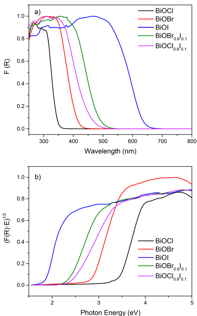
Fig. 4 a) DRUV-vis spectra and b) plots of transformed Kubelka-Munk function vs. photon energy (eV) of bismuth-based materials.
