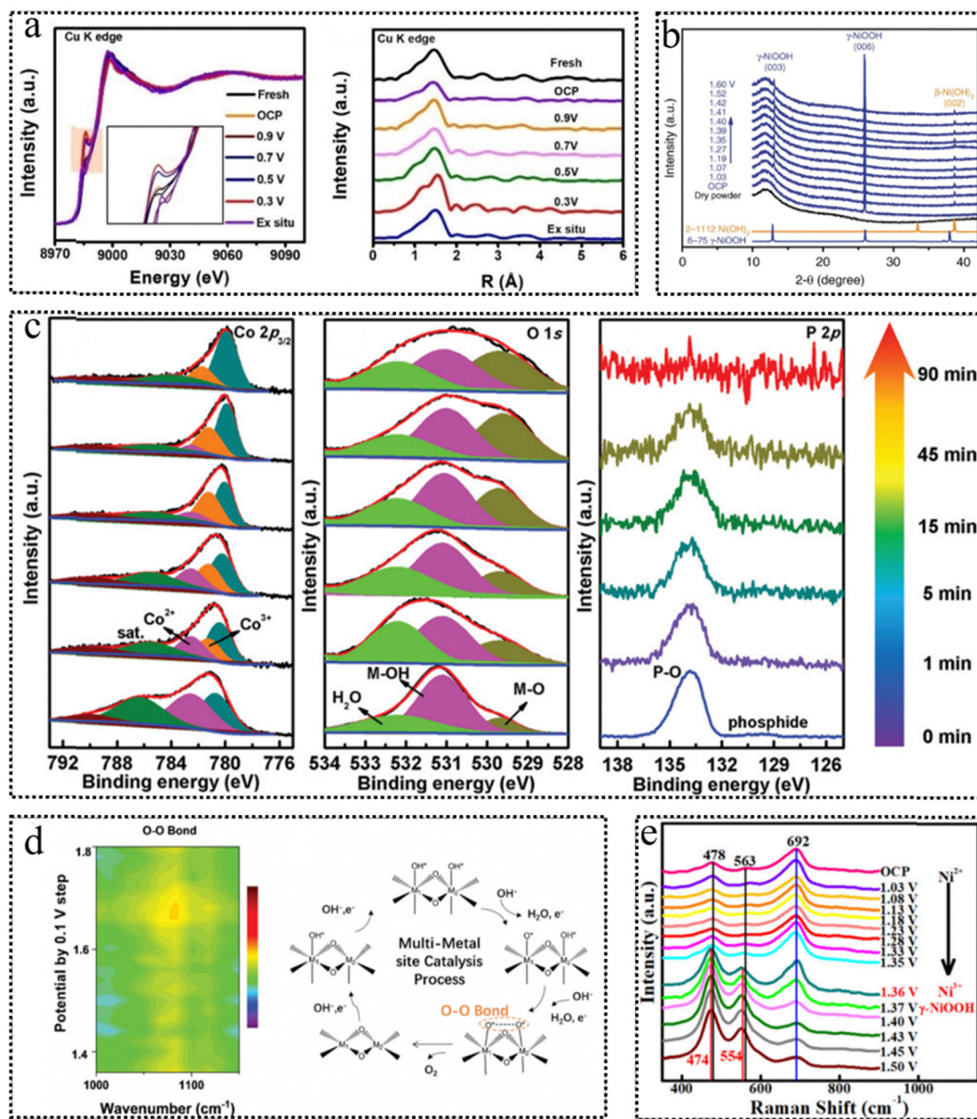
Fig. 6 (a) Operando Cu K-edge XAS spectra at different states and Cu K-edge FT-EXAFS spectra of Cu–N–C/GC. This figure has been reproduced from ref. 95 with permission from Wiley-VCH, copyright 2022. (b) Operando XRD patterns of \text{Ni(OH)}_2/\text{NF} at different potentials. This figure has been reproduced from ref. 96 with permission from Nature, copyright 2018. (c) Operando Co 2p 3/2 , O 1s and P 2p XPS spectra of \text{Co}_{0.8}\text{Fe}_{0.2}\text{P@C} . This figure has been reproduced from ref. 97 with permission from Wiley-VCH, copyright 2020. (d) 2D contour image of the operando ATR FT-IR spectrum for the OER (1.4–1.8 V vs. RHE) using 1 M KOH in \text{H}_2^{16}\text{O} and schematic illustration of the multi-metal-site catalytic mechanism. This figure has been reproduced from ref. 98 with permission from Royal Society of Chemistry, copyright 2020. (e) Operando Raman spectra of NFO/NF with photothermal effect ( i.e. , irradiated with 808-nm NIR light) from OCP to 1.50 V vs. RHE in 1.0 M KOH. This figure has been reproduced from ref. 99 with permission from American Chemical Society, copyright 2021.
