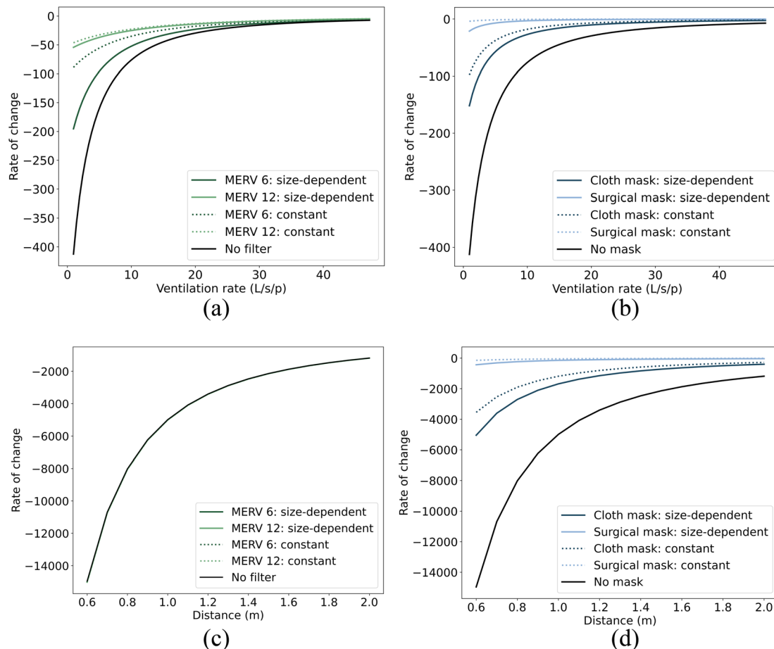
Fig. 4 Rate of change of virus concentration with ventilation/distancing for short-range airborne transmission when with constant and size-dependent efficiency of filters/masks and when without filters/masks. (a) Ventilation-filtration; (b) ventilation-mask; (c) distancing-filtration; (d) distancing-mask.
