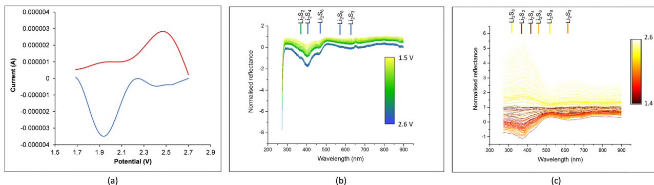
Fig. 5 Electrochemical test data from the first CV cycle of a Li-S battery cell: (a) CV curves in discharge (blue) and charge (red) at 0.041 \text{ mV s}^{-1} . In operando UV-vis spectra during (b) discharge and (c) charge, including the expected position for the absorbance peaks of the lithium sulfides.
