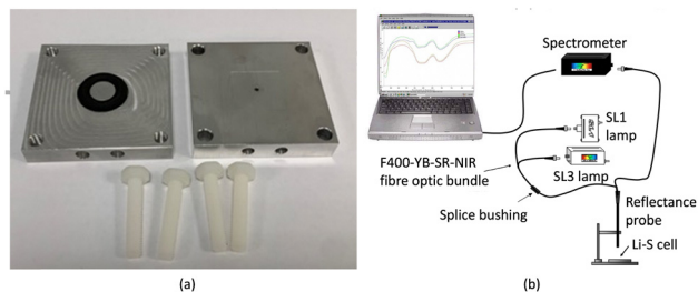
Fig. 4 Experimental set up for the Li-S battery testing: (a) three-part cell case with o-ring and top with a small hole in the middle under which a 25 \times 25 mm square quartz glass plate is placed over the battery cathode; (b) schematic diagram of the in operando UV-vis system monitoring a Li-S battery cell.
