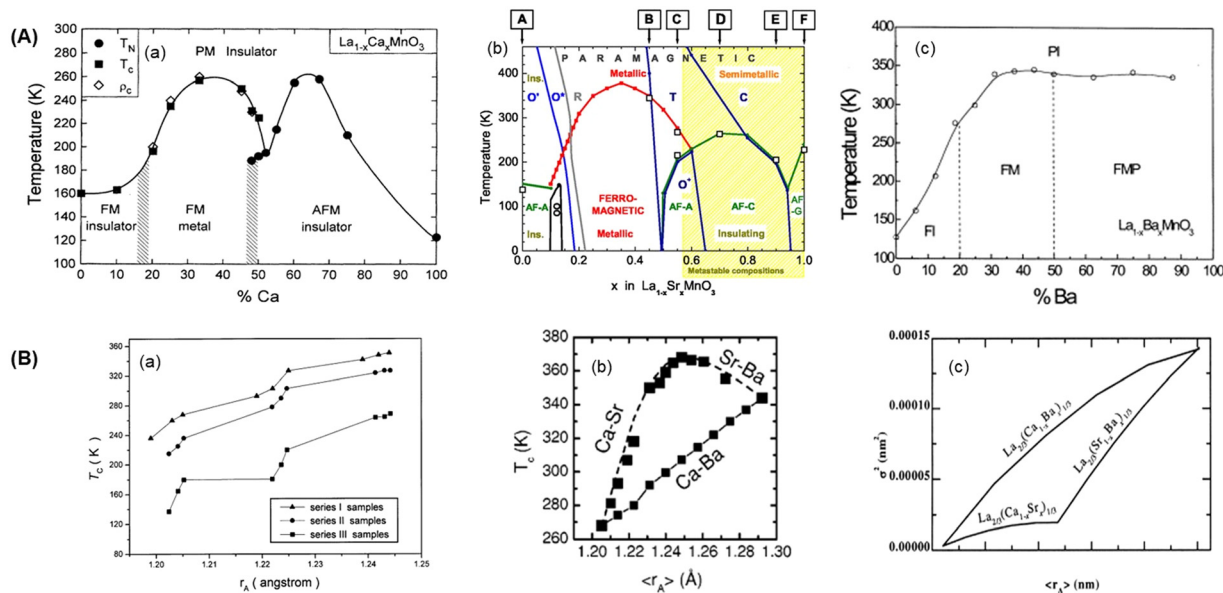
Fig. 6 Phase diagram of substituted PM materials in (A) (a) \text{La}_{1-x}\text{Ca}_x\text{MnO}_3 reprinted with permission, copyright 1995, American Physics Society, 154 (b) \text{La}_{1-x}\text{Sr}_x\text{MnO}_3 reprinted with permission, copyright 2005, American Physical Society, 157 (c) \text{La}_{1-x}\text{Ba}_x\text{MnO}_3 reprinted with permission, copyright 2000, Elsevier, 158 (B) graph of influencing \langle r_A \rangle to T_C reprinted with permission (a), copyright 2001, Elsevier, 159 (b), copyright 2002, American Institute of Physics 161 and (c) the influence \langle r_A \rangle to cation mismatch effect reprinted with permission, copyright 2002, Elsevier. 165
