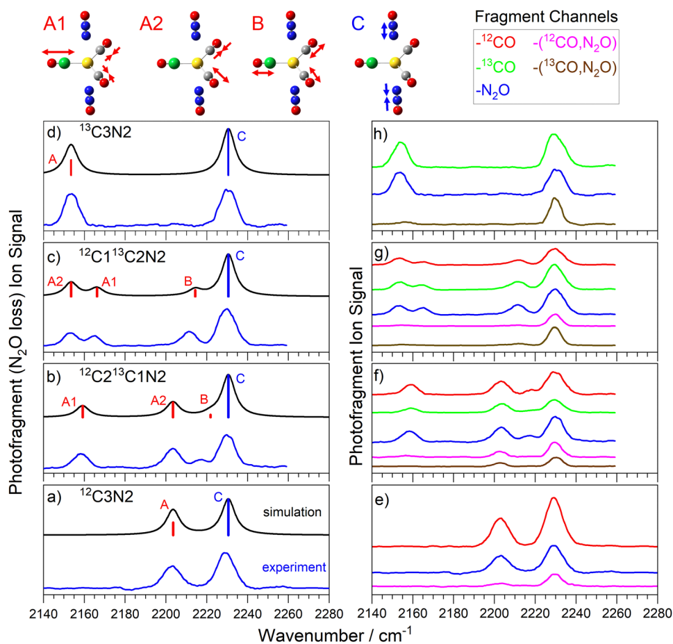
Fig. 4 (a)–(d) Comparison of experimental and simulated infrared action spectra of \text{Au}^{(12/13)\text{CO}}_3(\text{N}_2\text{O})_2^+ complexes, recorded in the \text{N}_2\text{O} loss channel. (e)–(h) Spectra recorded in different dissociation product channels, colour coded as above.
