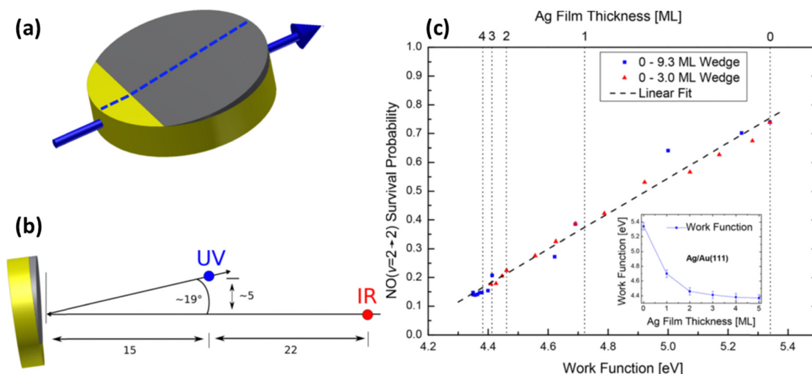
Fig. 11 Measurement of vibrational survival probability vs. systematically varied work function of the solid. (a) Wedged (not to scale) Ag thin film on Au(111). Film thickness is increasing when moving along the surface in the direction of the blue arrow. Scattering experiments have been performed along the center of the crystal (dashed line) enabling probing the locations with different work functions by the incident NO ( \nu = 2 ) molecular beam. (b) Positions of the UV REMPI (blue) and the IR-overtone pumping (red) beams relative to the surface and the molecular beam (represented by single-headed black arrows), used for quantification of vibrational survival probability. The laser beams are normal to the molecular beam and the surface normal. (c) Survival probability of NO ( \nu = 2 ) scattered from Ag/Au(111) plotted against the surface work function (see the inset for work function correlation with Ag film thickness). From ref. 83 with permission from American Chemical Society Copyright (2018).
