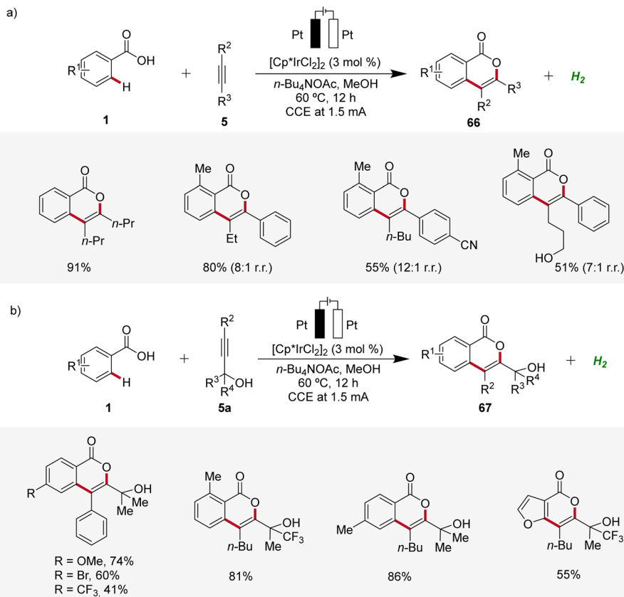
Scheme 19 Synthesis of isocoumarin derivatives 66 and 67 through irida-electrocatalysis.
