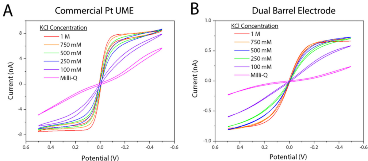
Fig. 6 Changes in voltammety with changing salt concentration on a (A) commercial CHI platinum UME ( r = 5 \mu\text{m} ) working electrode with a Pt wire quasi-reference counter electrode and (B) a dual barrel electrode (WE r = 0.59 \mu\text{m} , QRCE r = 0.60 \mu\text{m} ). Voltammety was taken in a 5 mM potassium hexacyanoferrate(II/III) solution with changing salt concentration from 0.5 V to -0.5 V at a scan rate of 0.1 \text{ V s}^{-1} with a 2 seconds quiet time for 5 scans. The final scan for each voltammogram is plotted in polarographic convention.
