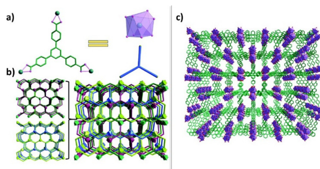
Fig. 6 (a) The coordination environments of Eu 3+ and H 3 BTB. (b) The topology structure of MHT-1 with a [2 + 2] mode. (c) The 3D four-fold interpenetrated framework of MHT-1 . Reproduced from ref. 78 with permission from Royal Society of Chemistry, copyright 2019.
