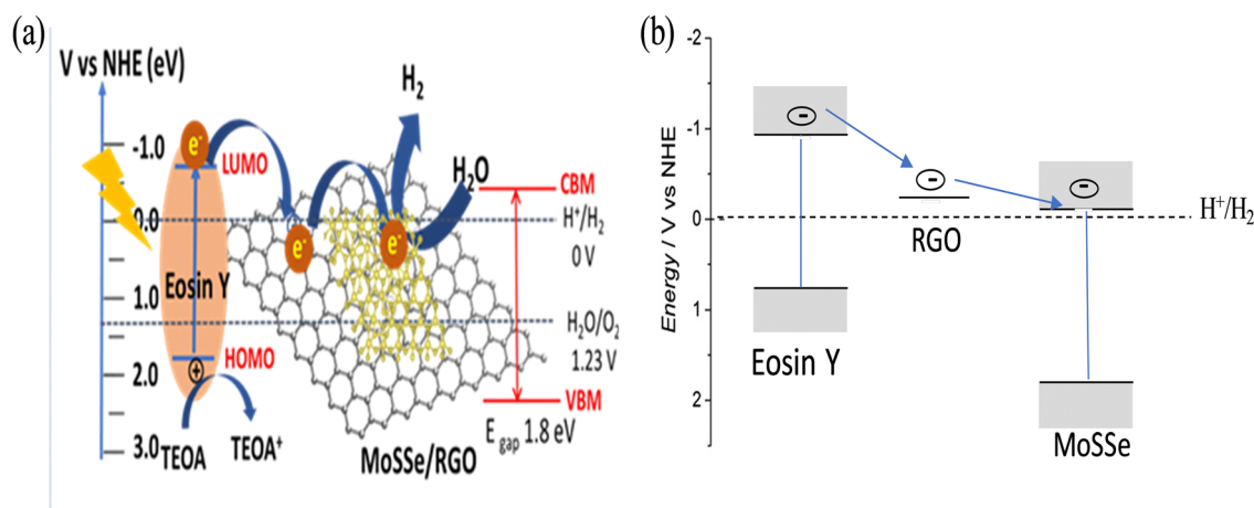
Fig. 8 (a) and (b) A schematic illustration representing the dye-sensitized photocatalytic HER mechanism of the MoSSe@RGO nanocomposites using TEAO sacrificial agent under visible-light irradiation. VBM (valence band minimum); CBM (conduction band maximum); HOMO (highest occupied molecular orbital); LUMO (lowest unoccupied molecular orbital).
