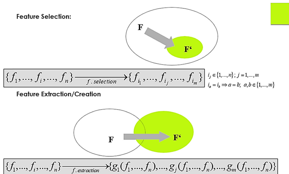
Fig. 12 Illustration of difference between feature selection and feature extraction.
