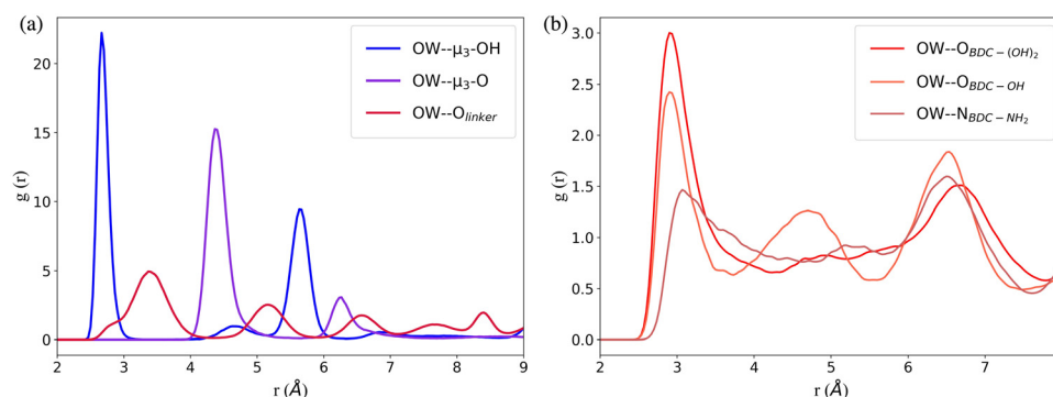
Fig. 2 The radial distribution function (RDF) between the oxygen of water (OW) and the oxygen or nitrogen atoms in (a) the \mu_3 -OH, \mu_3 -O and O_{\text{linker}} interaction sites in UiO-66 and (b) in the -\text{NH}_2 and -\text{OH} functional groups in the three functionalized derivatives of UiO-66. All plots were obtained from simulations with the same number of water molecules per unit cell as UiO-66 at 10% relative humidity (RH).
