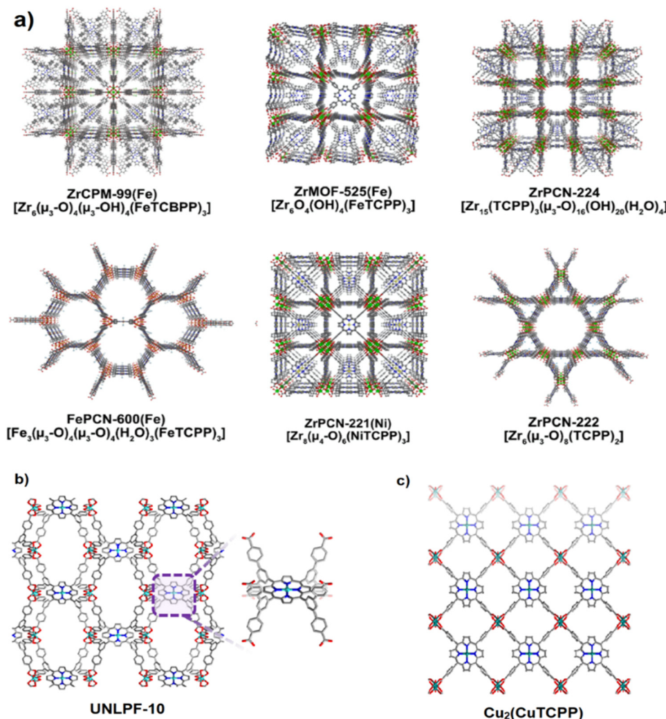
Fig. 17 Porphyrin-based MOFs can be transformed into PC functional materials. Color scheme: Zr (green); Fe (orange); Ni (yellow); O (red); N (blue); C (grey). Structure of UNLPPF-10 featuring in-porphyrin sites for the photocatalytic oxidation of thioanisole (b). Structure of \text{Cu}_2(\text{CuTCPP}) featuring \text{Cu}_2 nodes and Cu-porphyrin sites for the electrochemical reduction of \text{CO}_2 to formate and acetate (c). Reproduced from ref. 140 and 141 with permission with Elsevier.
