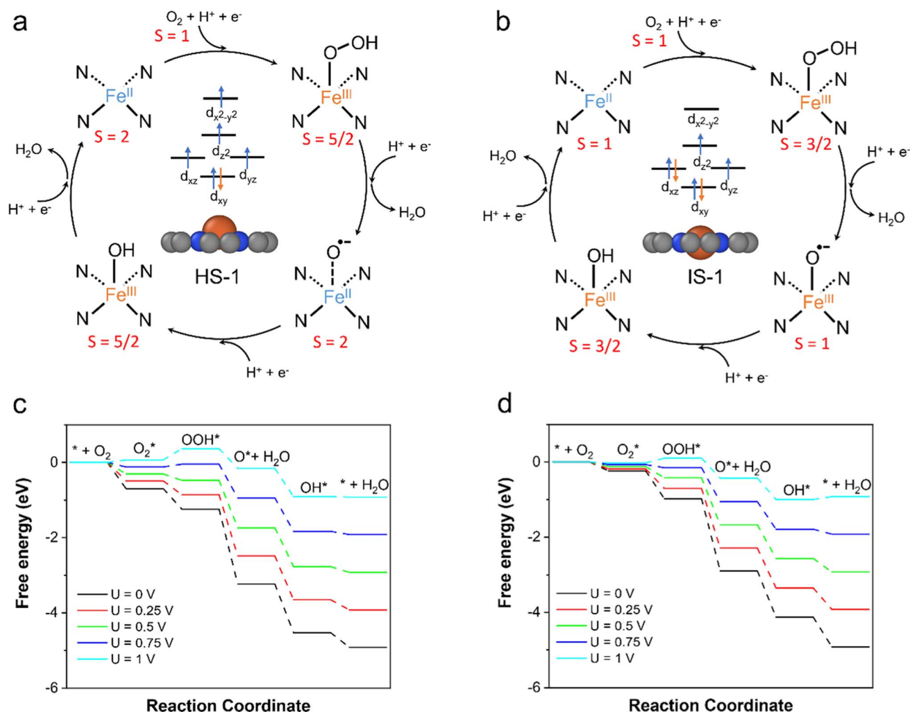
Fig. 6 Proposed spin-dependent ORR mechanism on FeN 4 C 10 . (a) High-spin ORR cycle. (b) Intermediate-spin ORR cycle. (c) High-spin ORR free energy diagram. (d) Intermediate-spin ORR free energy diagram.
