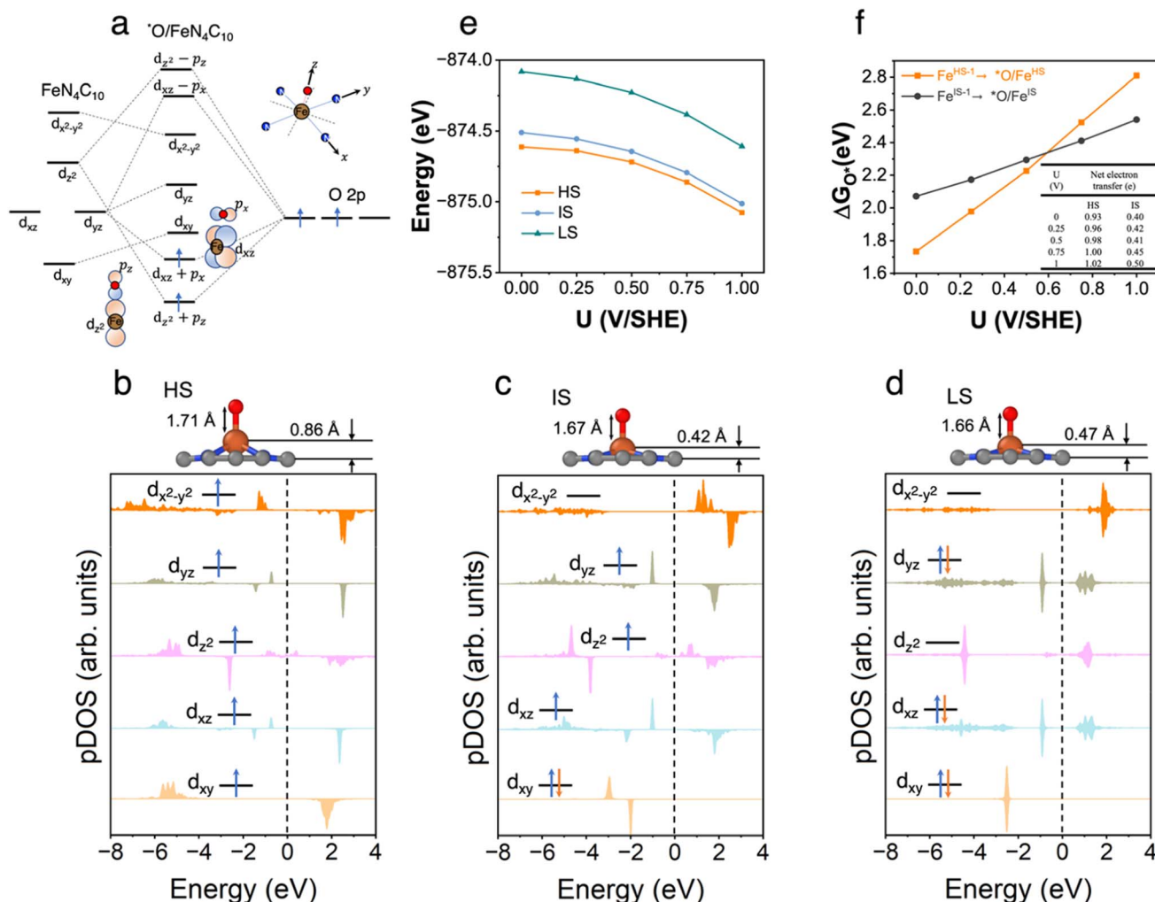
Fig. 4 ^*\text{O}/\text{FeN}_4\text{C}_{10} . (a) Schematics of orbital hybridizations of Fe 3d orbitals in a square-planar ligand field with the 2p orbitals in the O adsorbate. (b)–(d) Atomic structures and pDOS plots of the HS, IS, and LS states of ^*\text{O}/\text{FeN}_4\text{C}_{10} . (e) Spin- and potential-dependent energies of ^*\text{O}/\text{FeN}_4\text{C}_{10} under constant-potential conditions. (f) Spin and potential-dependent ^*\text{O} adsorption energies. The inset table shows the net electron transfer in the adsorption process.
