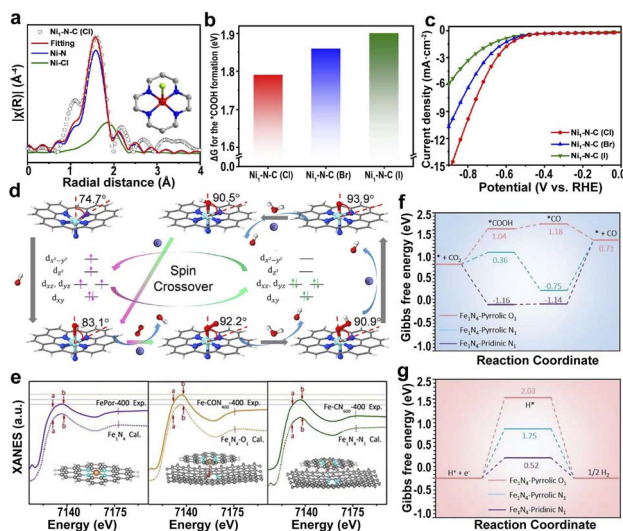
Fig. 9 (a) EXAFS fitting of \text{Ni}_1\text{-N-C(Cl)} . (b) The \Delta G for the \text{*COOH} formation in \text{Ni}_1\text{-N-C(X)} catalysts. (c) LSV curves of \text{Ni}_1\text{-N-C(X)} . 181 Copyright 2022, Springer. (d) Structure and dynamics of the N– \text{FeN}_4\text{C}_{10} moiety in the ORR with optimized geometries (the angles represent the deviation of iron from the \text{N}_4 -plane). 184 Copyright 2020, Elsevier. (e) Experimental XANES curves and the calculated XANES data for \text{Fe}_1\text{N}_4 (FePor-400, by calcinating iron porphyrin at 400 °C), \text{Fe}_1\text{N}_4\text{-O}_1 (Fe-CON 400 -400, by calcinating O, N codoped carbon at 400 °C to form \text{CON}_{400} , and loading iron porphyrin on \text{CON}_{400} at 400 °C to fabricate Fe-CON 400 -400), and \text{Fe}_1\text{N}_4\text{-N}_1 (Fe-CN 600 -400, by calcinating O, N codoped carbon at 600 °C under 5% \text{H}_2/\text{Ar} to form \text{CN}_{600} , and loading iron porphyrin on \text{CN}_{600} at 400 °C to fabricate Fe-CN 600 -400). Gibbs free energy diagrams for the (f) \text{CO}_2\text{RR} and (g) HER pathways on Fe sites of different configurations. 185 Copyright 2021, The Royal Society of Chemistry.
